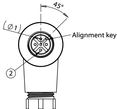
Front View Not to Scale
