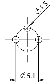
PCB Layout
