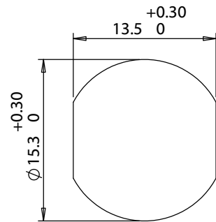
Panel cutout (PG9) Panel thickness (4.5mm max.)
