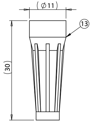
Strain relief
