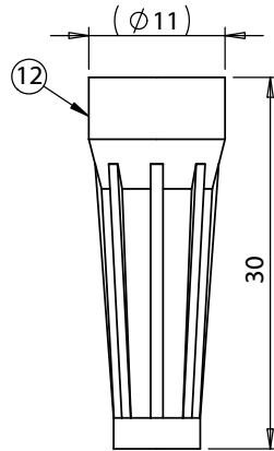
Strain relief
