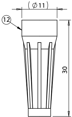
Strain relief
