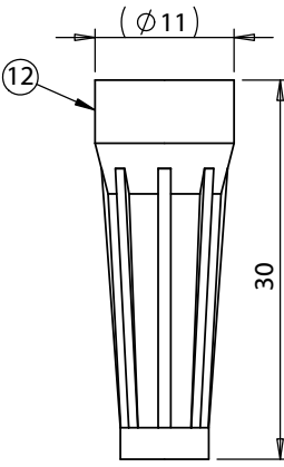
Strain relief
