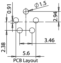
PCB Layout
