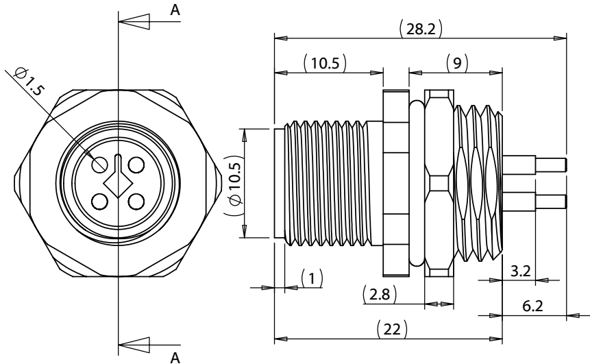
Panel cutout (M16 x 1.5) Panel thickness (4.5mm max.)
